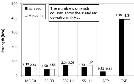
Figure 3. Strength and standard deviation of sprayed and mixed-in specimens
