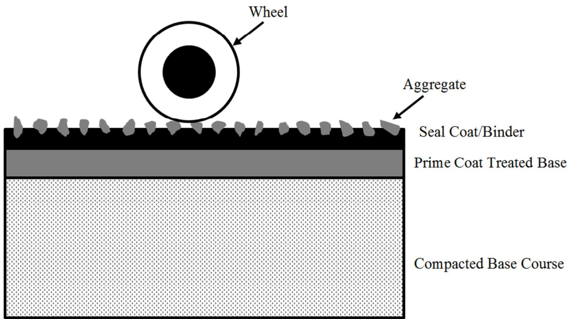
Figure 1. Typical pavement section after prime coat and pavement application
