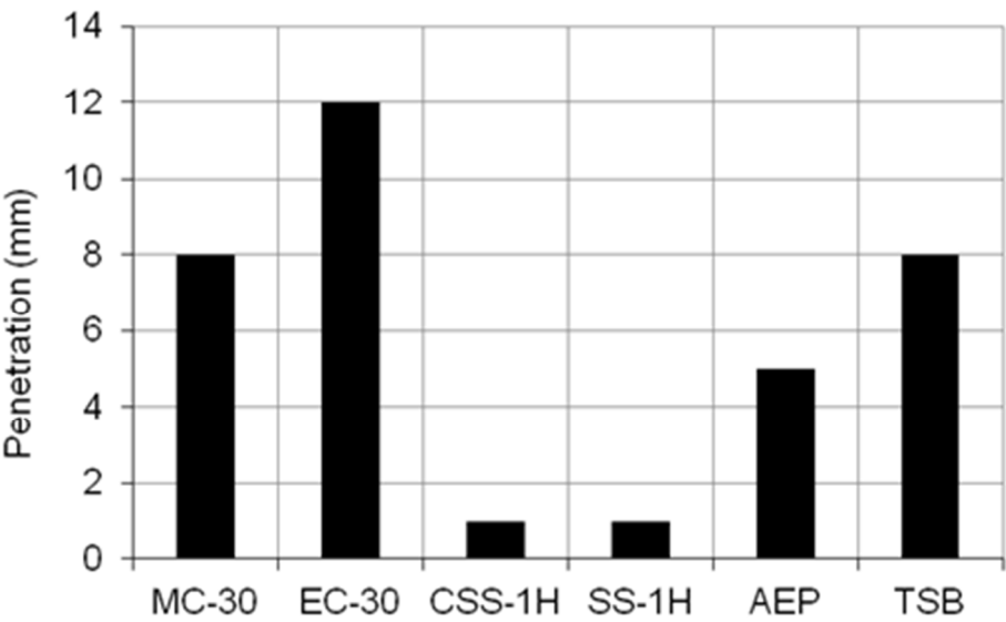
Figure 5 Penetration values measured for different prime coats.
