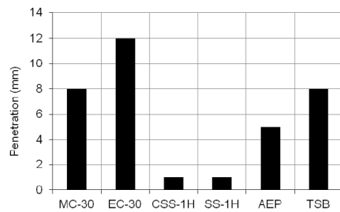
Figure 5. Penetration values measured for different prime coats.
