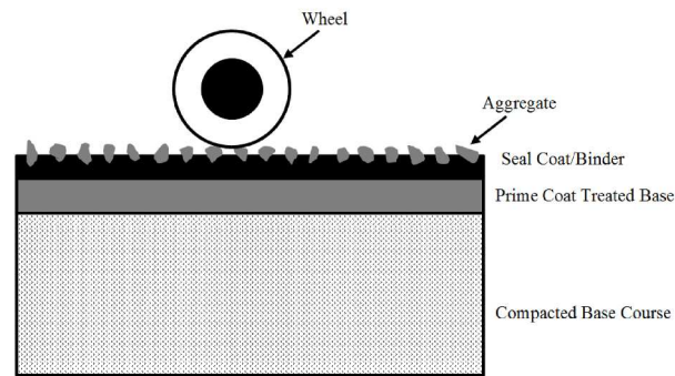
Figure 1. Typical pavement section after prime coat and pavement application
