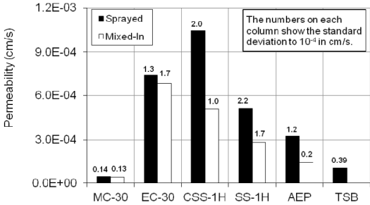
Figure 4. Permeability and standard deviation values of sprayed and mixed-in prime coat materials
